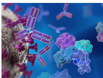
Fig. 1 Schematic diagram of antibody action.
