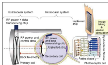
Fig. 2 Retinal prosthesis device
