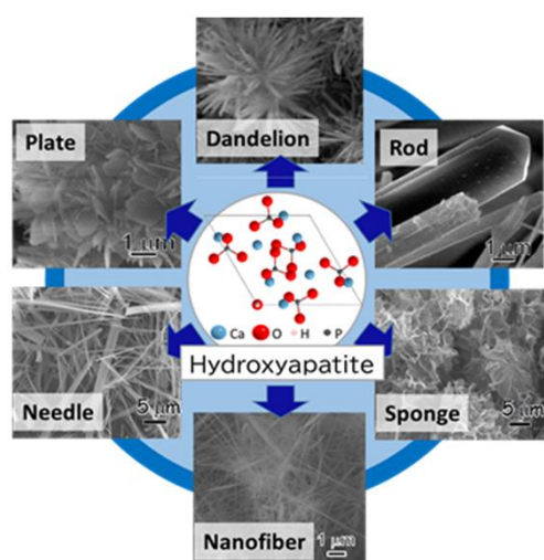
Fig. 1 Crystal morphology of hydroxyapatite synthesized by hydrothermal method
