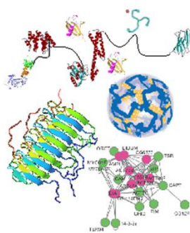
Fig.2 Biological complex molecular systems
